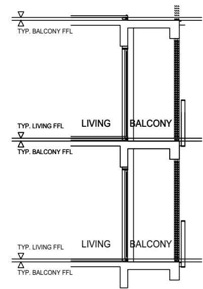
TYPICAL RETRACTABLE BALCONY SCREEN - SECTION AA
