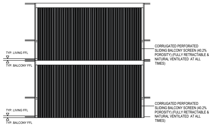
TYPICAL RETRACTABLE BALCONY SCREEN (CLOSED) - ELEVATION 1
