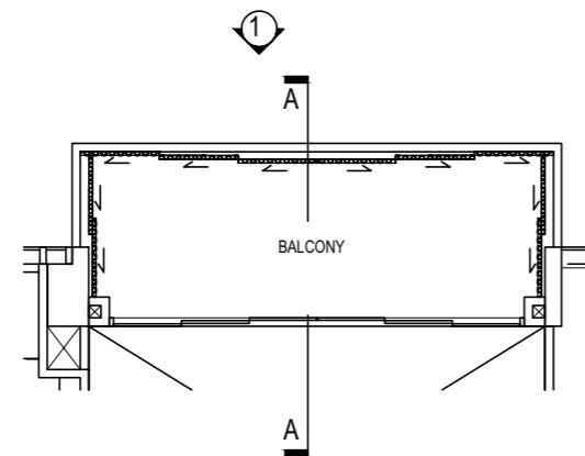
TYPICAL RETRACTABLE BALCONY SCREEN (FULLY CLOSED) - PLAN
